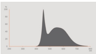
LISO spectral power distribution 6500K CRI80 v1
